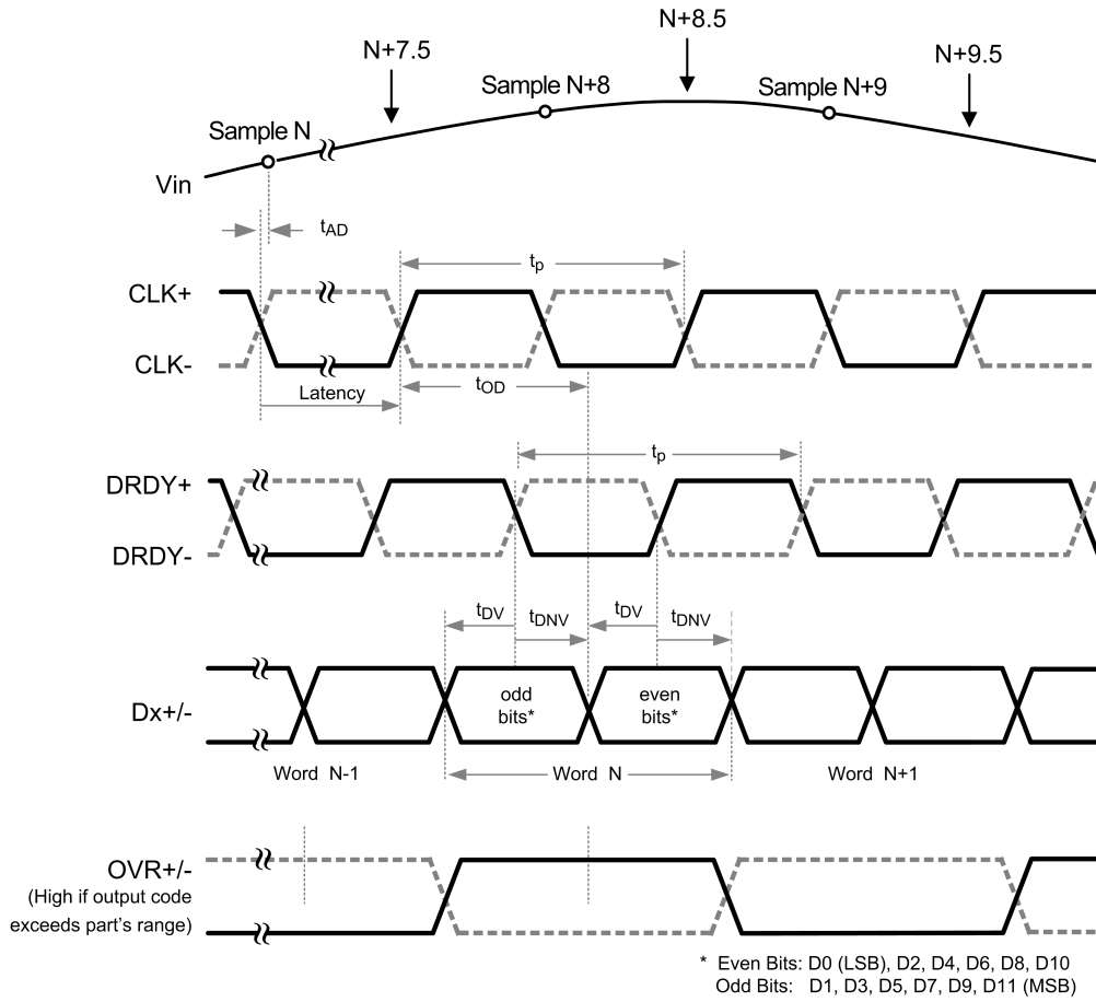
Output Timing
